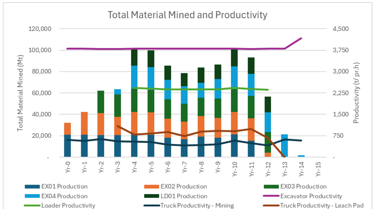
Figure 1-8 Total material mined and productivity
