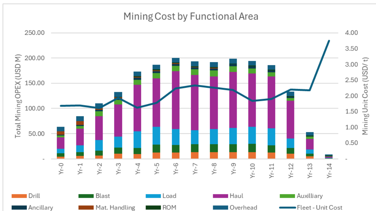
Figure 1-13 Mining cost by functional area
